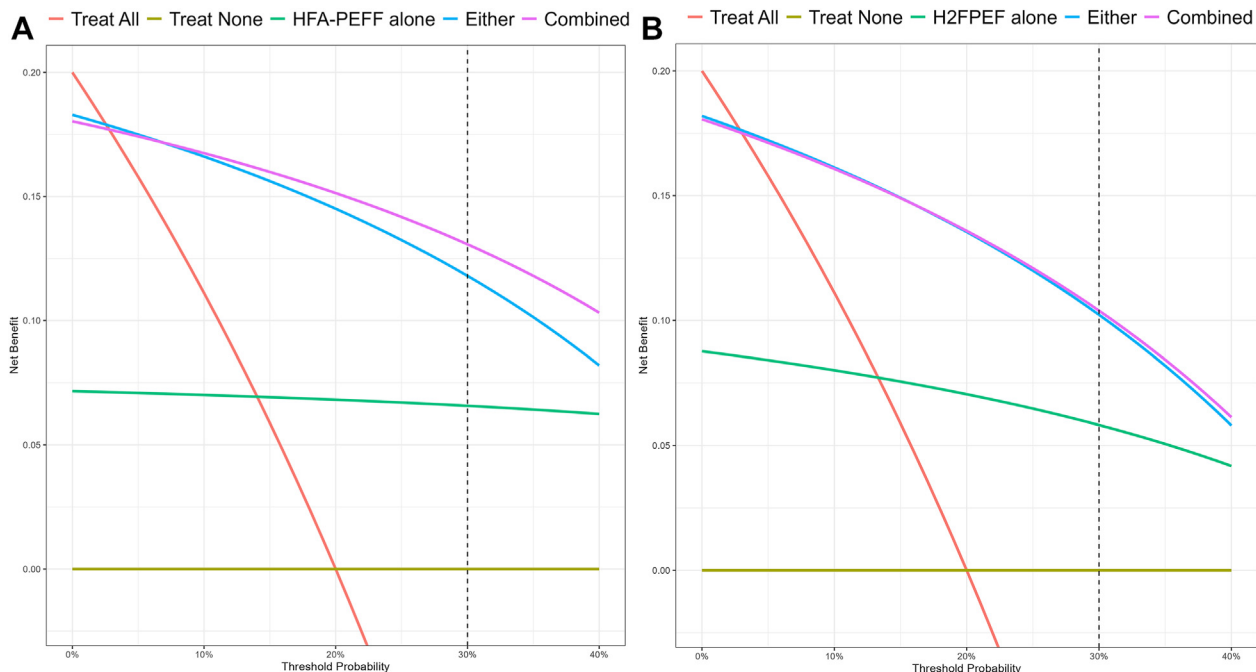
FIGURE 4 Decision Curve Analysis for Patient Management Decisions Incorporating the AI HFpEF Model
